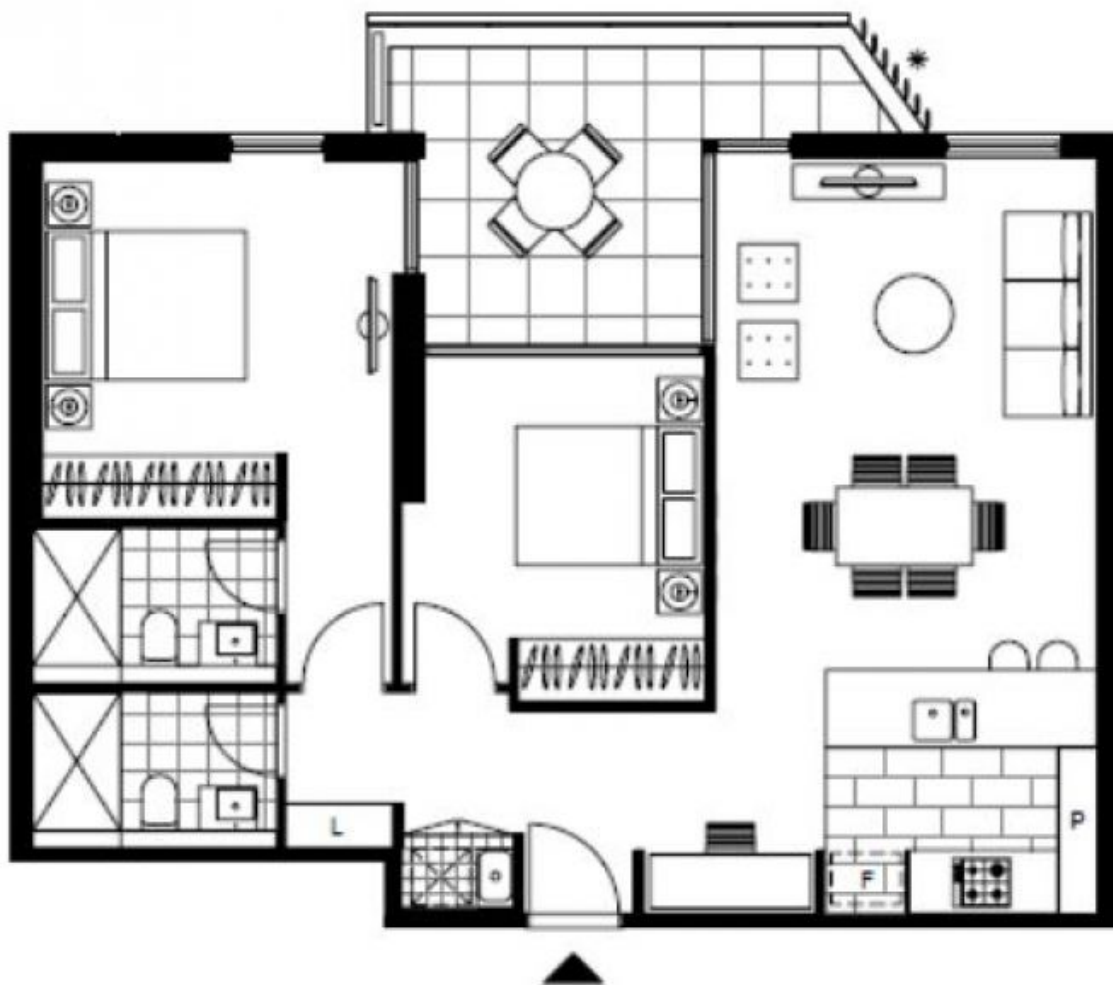
LEVEL 3
