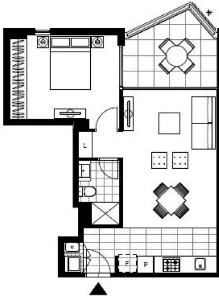
LEVEL 2, 4
