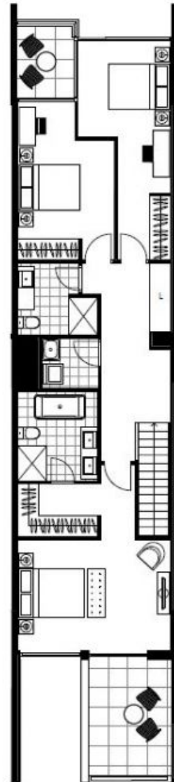
SECOND FLOOR
